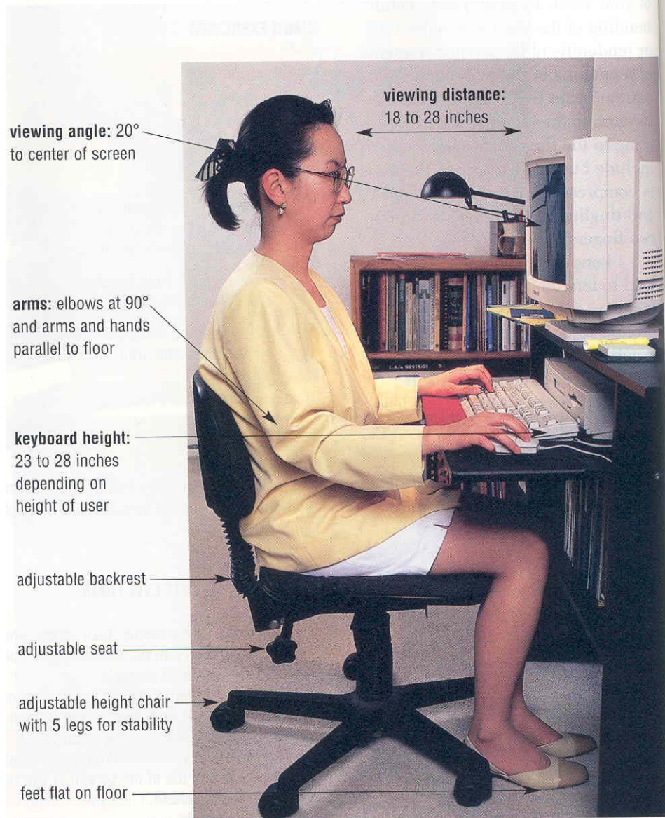
Figure 11-43 A well-designed work area should be flexible to allow adjustments to the height and build of different individuals. Good lighting and air quality also are important considerations.
